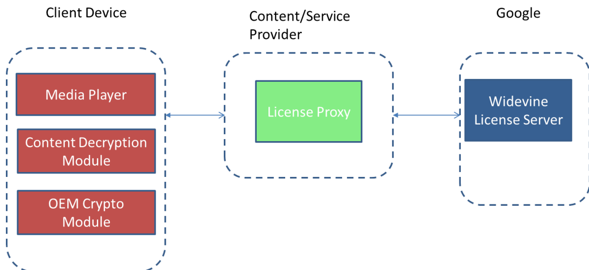
Figure 4: Widevine DRM Architecture
