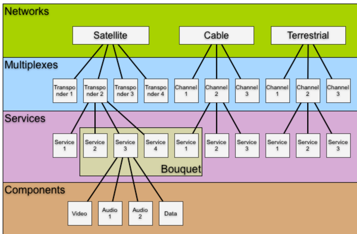
Figure 2: Service delivery model
