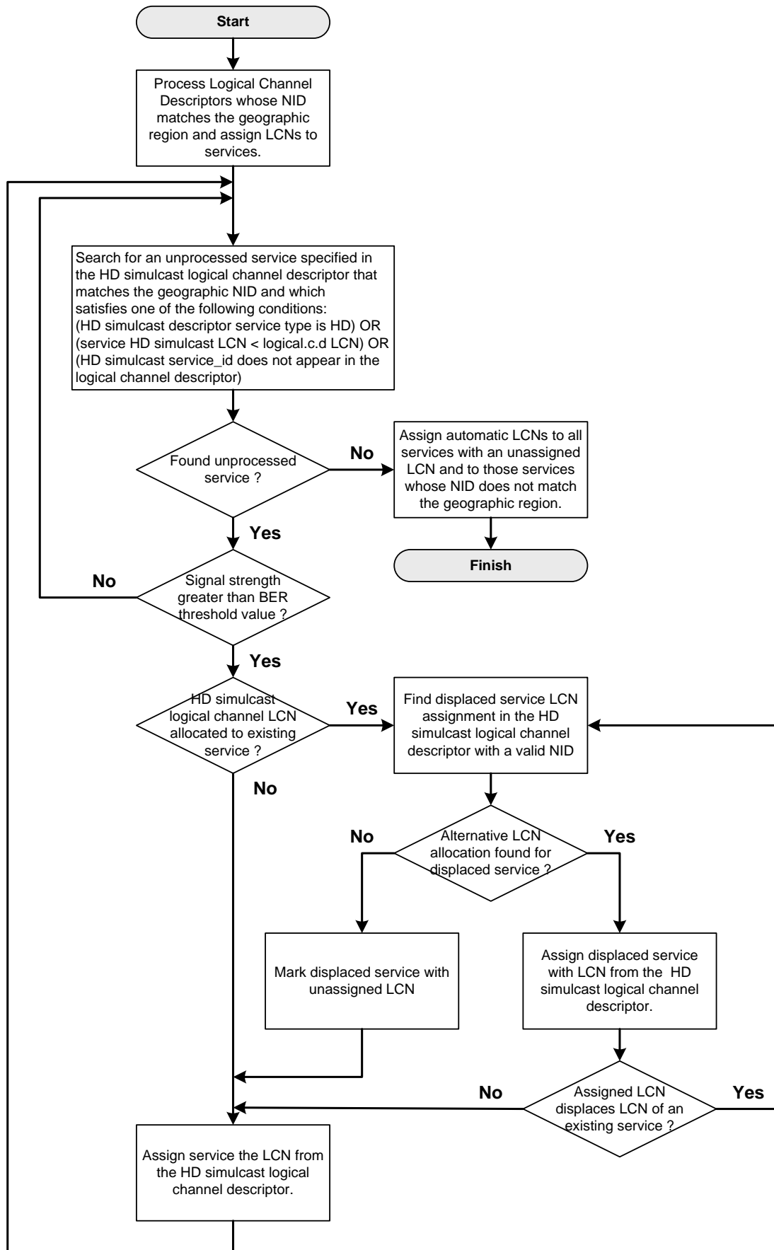
Figure 1: HD_simulcast_LCN operation
