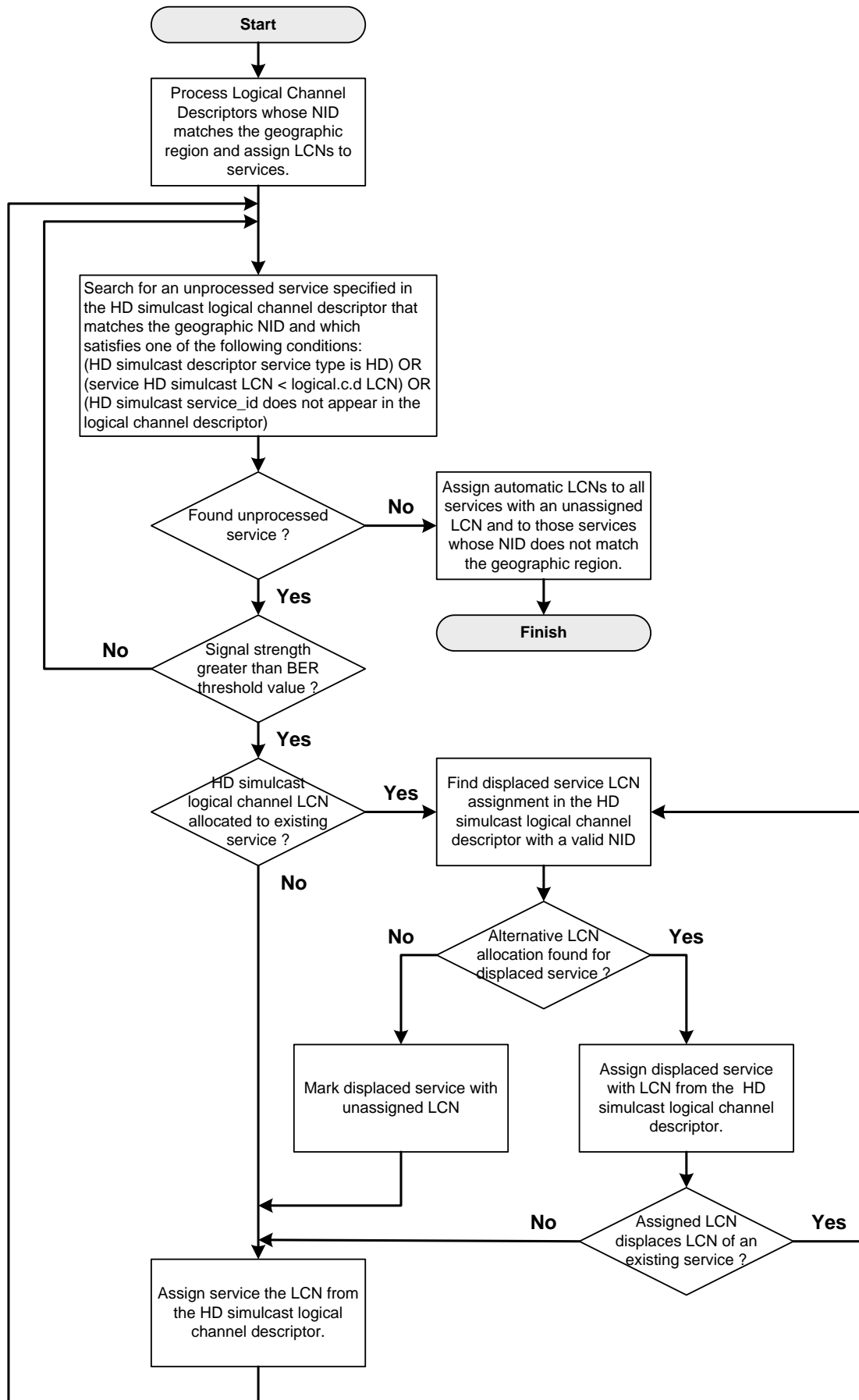
Figure 1: HD_simulcast_LCN operation
