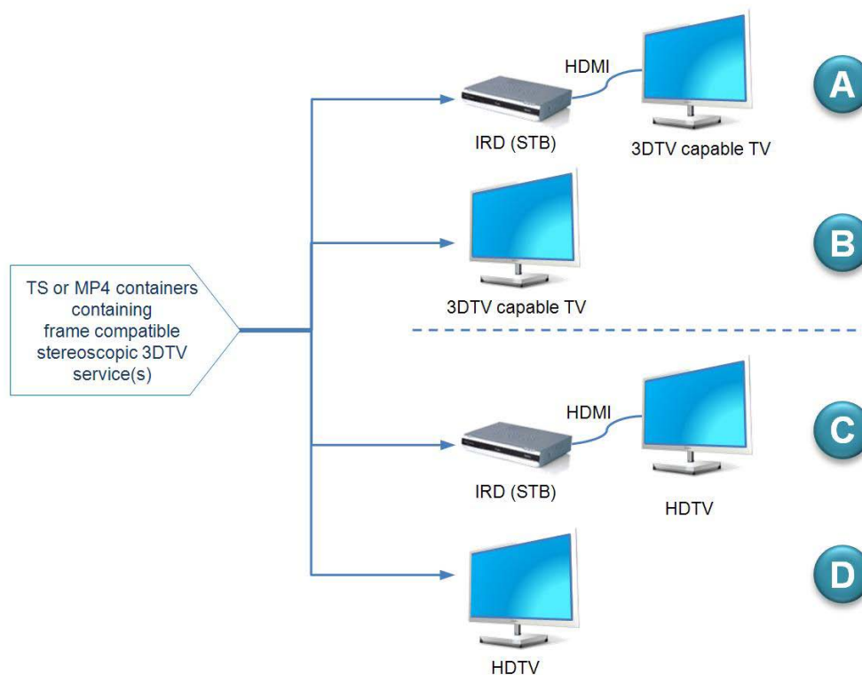
Figure 14: Frame compatible plano-stereoscopic 3DTV IRD use cases
