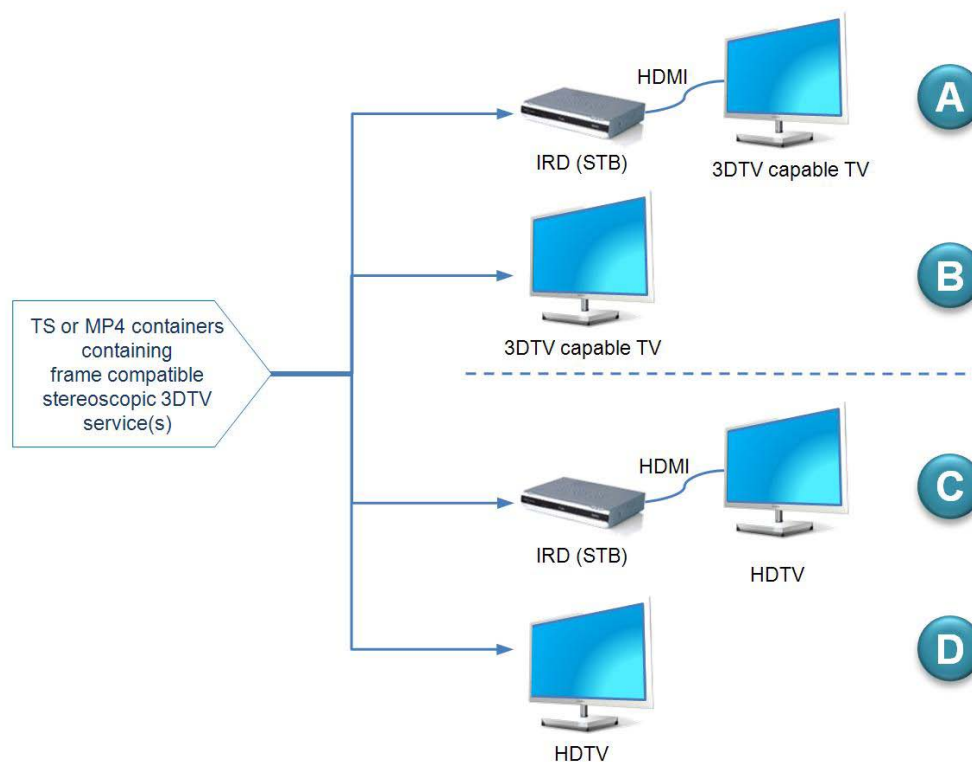
Figure 16: Frame compatible plano-stereoscopic 3DTV IRD use cases
